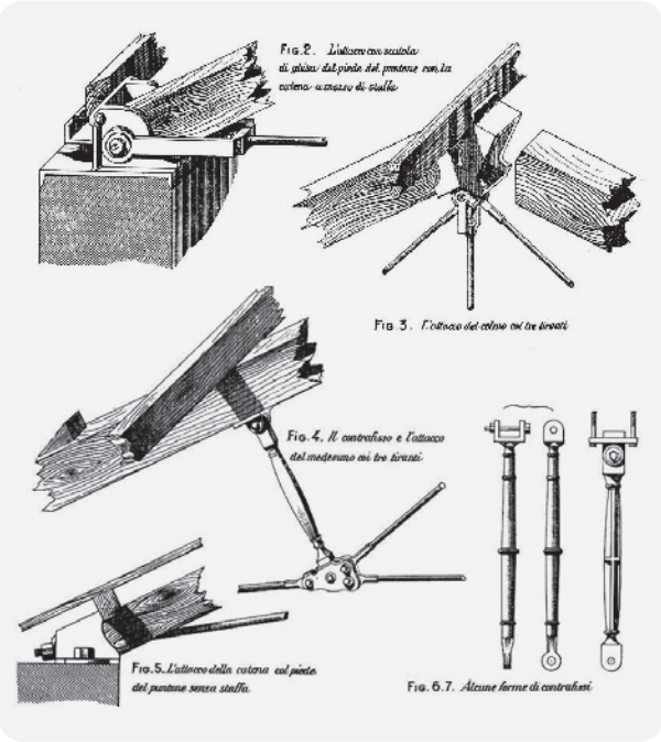
Wooden truss tie rods
